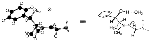
Figure 5. Crystal structure of pseudoephedrine glycinamide monohydrate.
